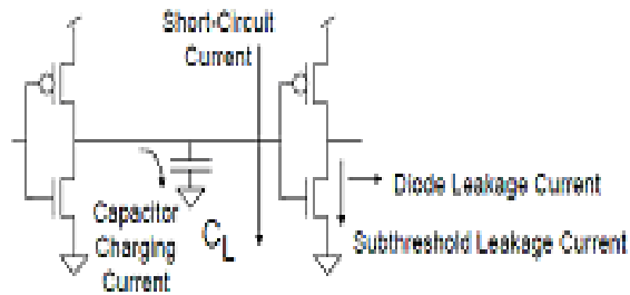
Figure 2, Power Dissipation in CMOS [4]
